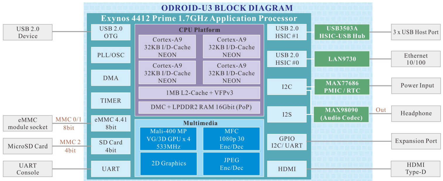
A block diagram showing the architecture of the ODROID-U3.
