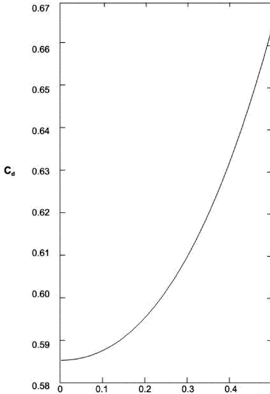
FIGURE 13. Variation of C_d for 90^\circ V-Notch weir with H^2/A
