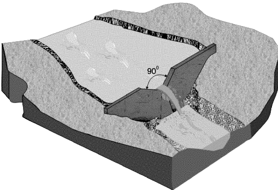
FIGURE 12. General view of 90° v-notch weir
