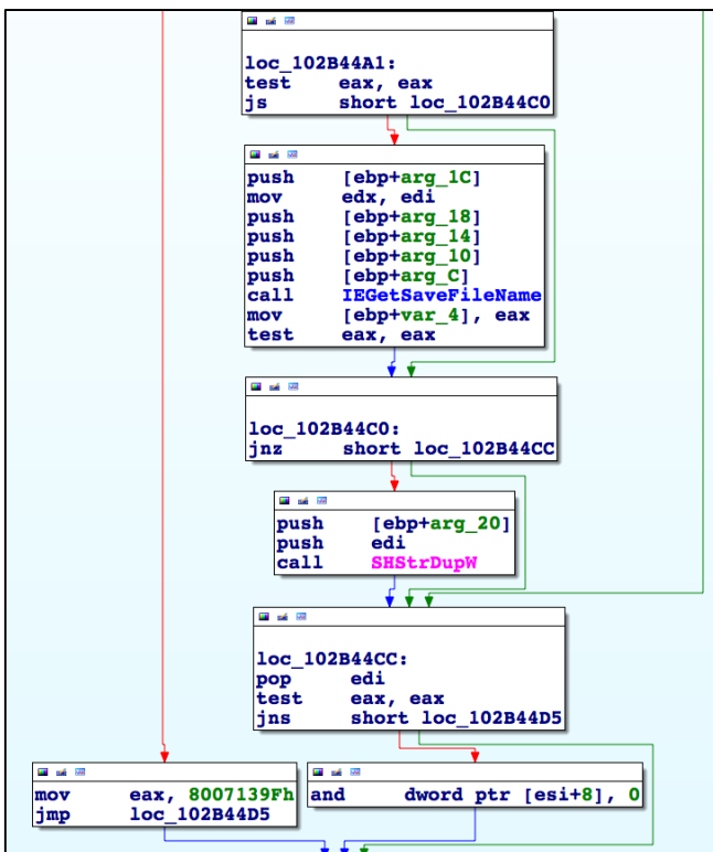
Figure 11 Pre-patch code
