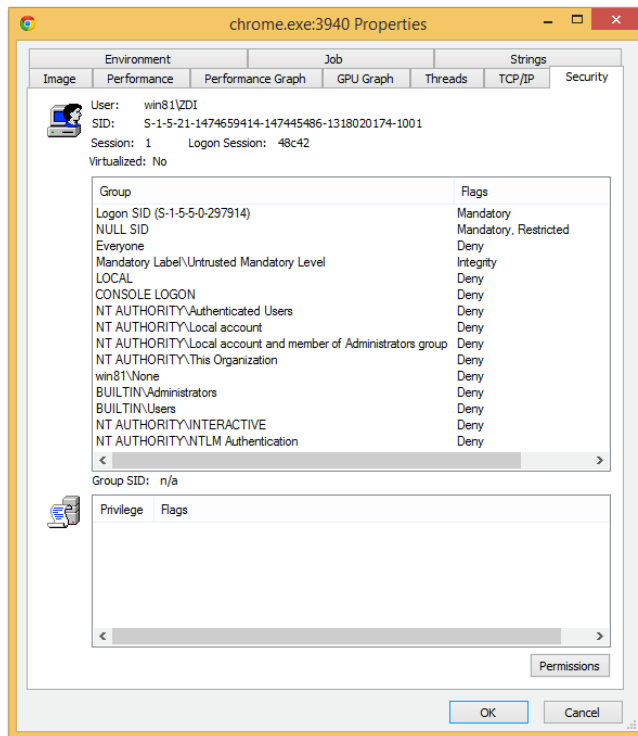
Figure 2 Google Chrome restrictions
