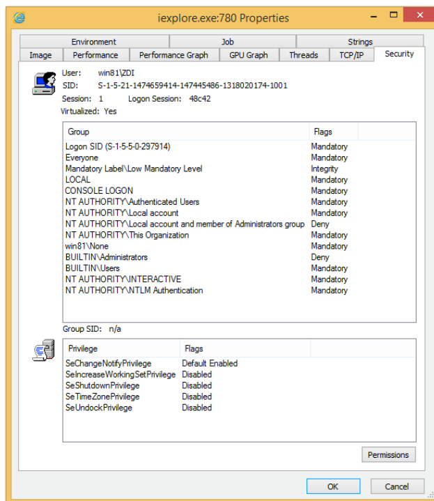
Figure 1 Microsoft Internet Explorer restrictions
