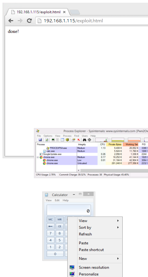
Figure 14 Sandbox escape using MoreOlePrivateData
