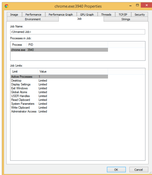
Figure 3 Google Chrome Job Object Limitations
