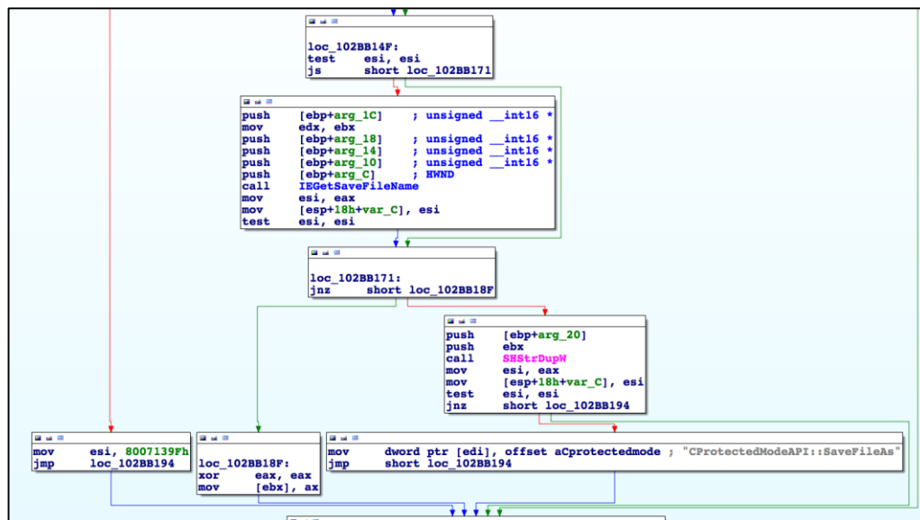
Figure 12 Post-patch code
